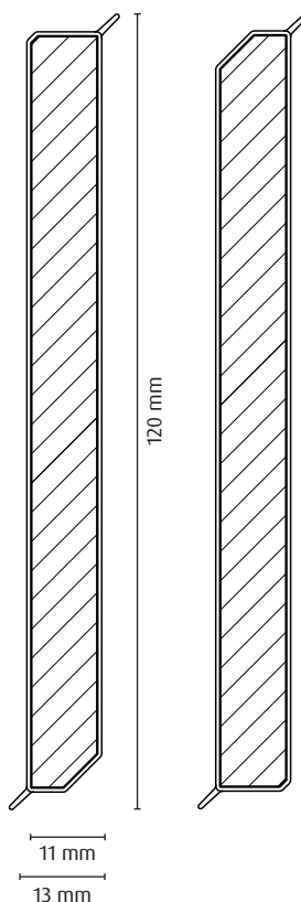
FN TURN-X120 11 x 120 x 2400 mm
