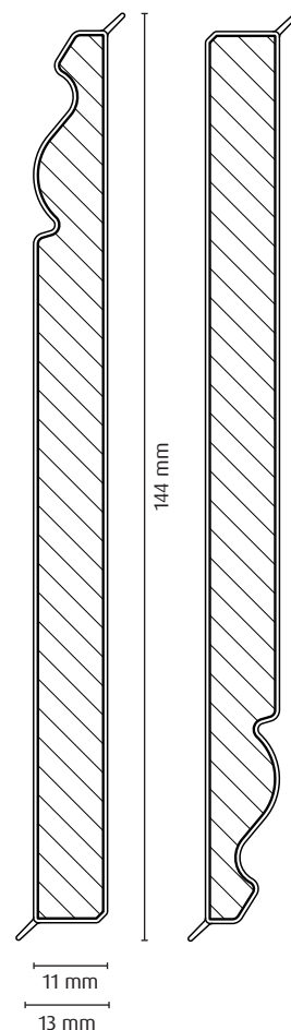
FN SWING-X144 11 x 144 x 2400 mm
